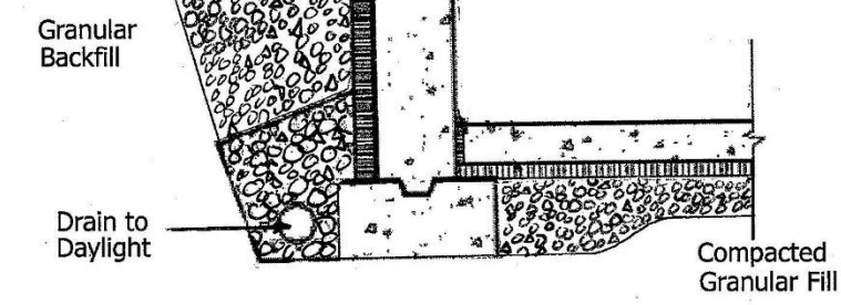
WALL SECTION - TYP.
